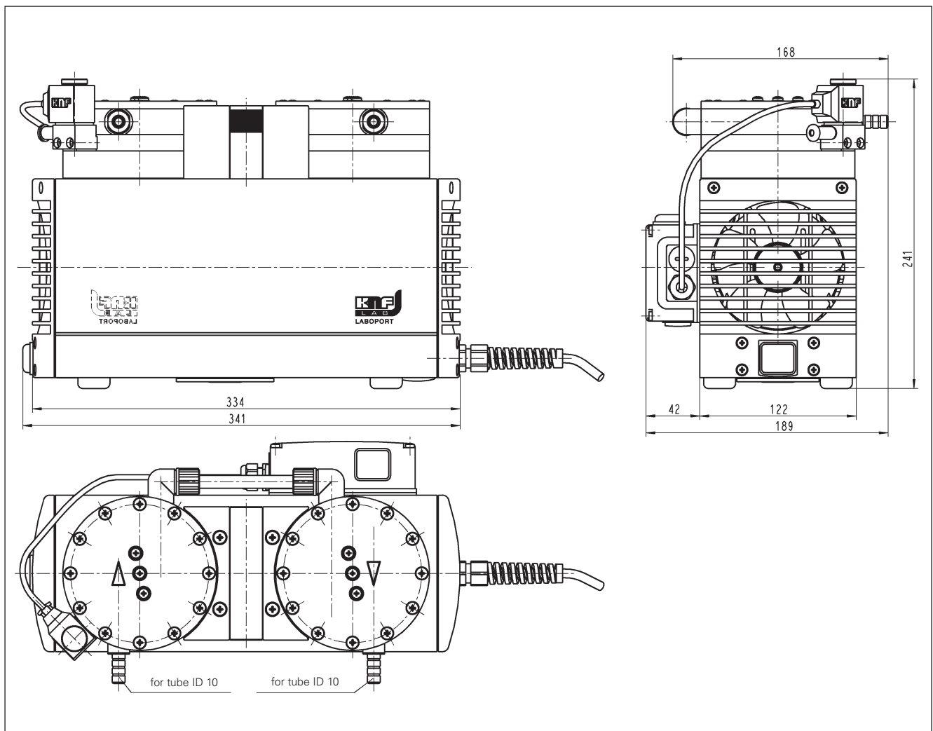
Dimensions (mm)
